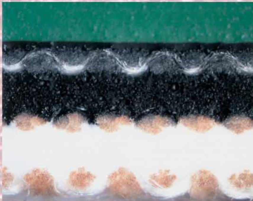
Cross cut of the 3-ply Perfect Dot® DL
